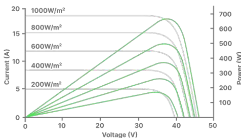
I-V Curves Of PV Module
